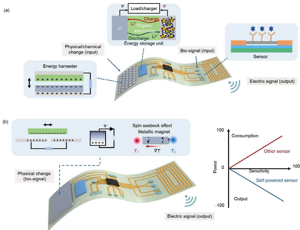
Fig. 1. Schematics of the two main modes of self-powered technology for the next generation of biosensors. (a) The self-powered sensing system based on an energy-harvesting unit. (b) The self-powered sensor based on the direct conversion of chemical/physical environmental changes.
